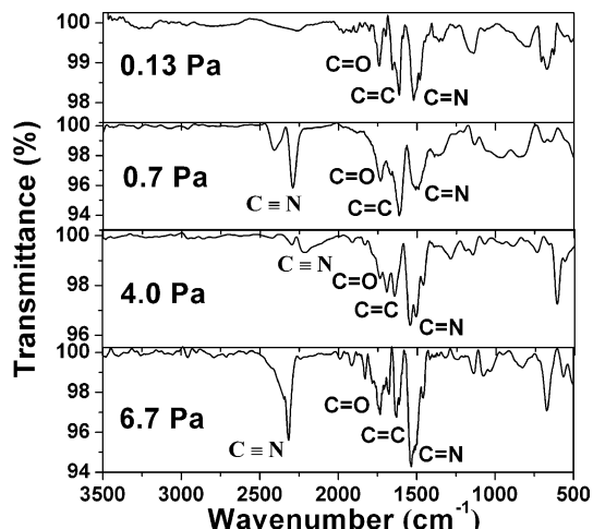
Fig. 6. FTIR analyses of CN x thin films deposited by PLD of graphite at 300 °C, 10 J/cm 2 , and at the indicated nitrogen pressures.
