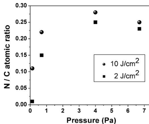
Fig. 5. XPS N 1s/C 1s peak area ratio, qualitatively indicating the N concentration, as a function of nitrogen gas pressure for CN x thin films deposited by PLD of graphite at 10 and 2 J/cm 2 .
