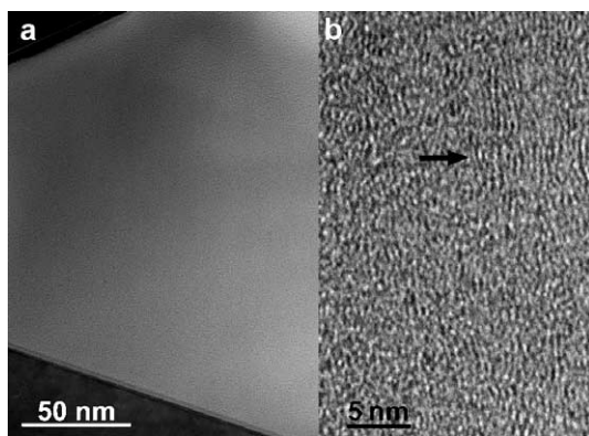
Fig. 1. Cross-sectional TEM micrographs of a CN_x thin film deposited by PLD of graphite on a Si (100) substrate at 300 °C, 10 J/cm 2 and 0.13 Pa N 2 . (a) represents an overview and (b) high-resolution image from the regions containing bundles of corrugated graphene planes (marked by an arrow).
