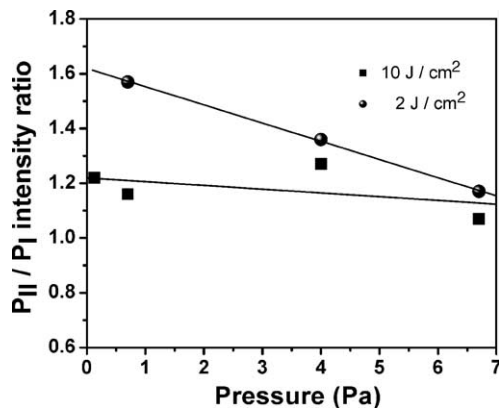
Fig. 3. Variation of the intensity ratio P_{II}/P_I as a function of gas pressure, for two different laser fluences: 2 and 10 J/cm 2 , where peaks I (398 eV) and II (400 eV) are the main components of N 1s core level spectra.
