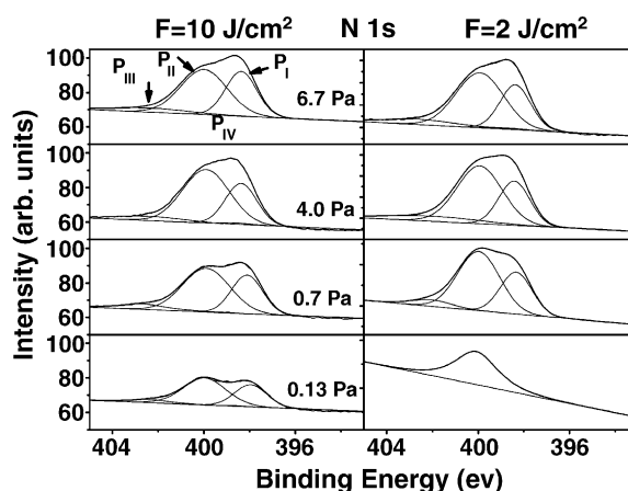
Fig. 2. XPS N 1s core level spectra of CN_x thin films deposited by PLD of graphite at the indicated pressures and fluences.
