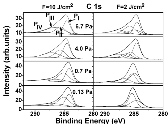
Fig. 4. XPS C 1s core level spectra of CN x thin films deposited by PLD of graphite at the indicated pressures and fluences.
